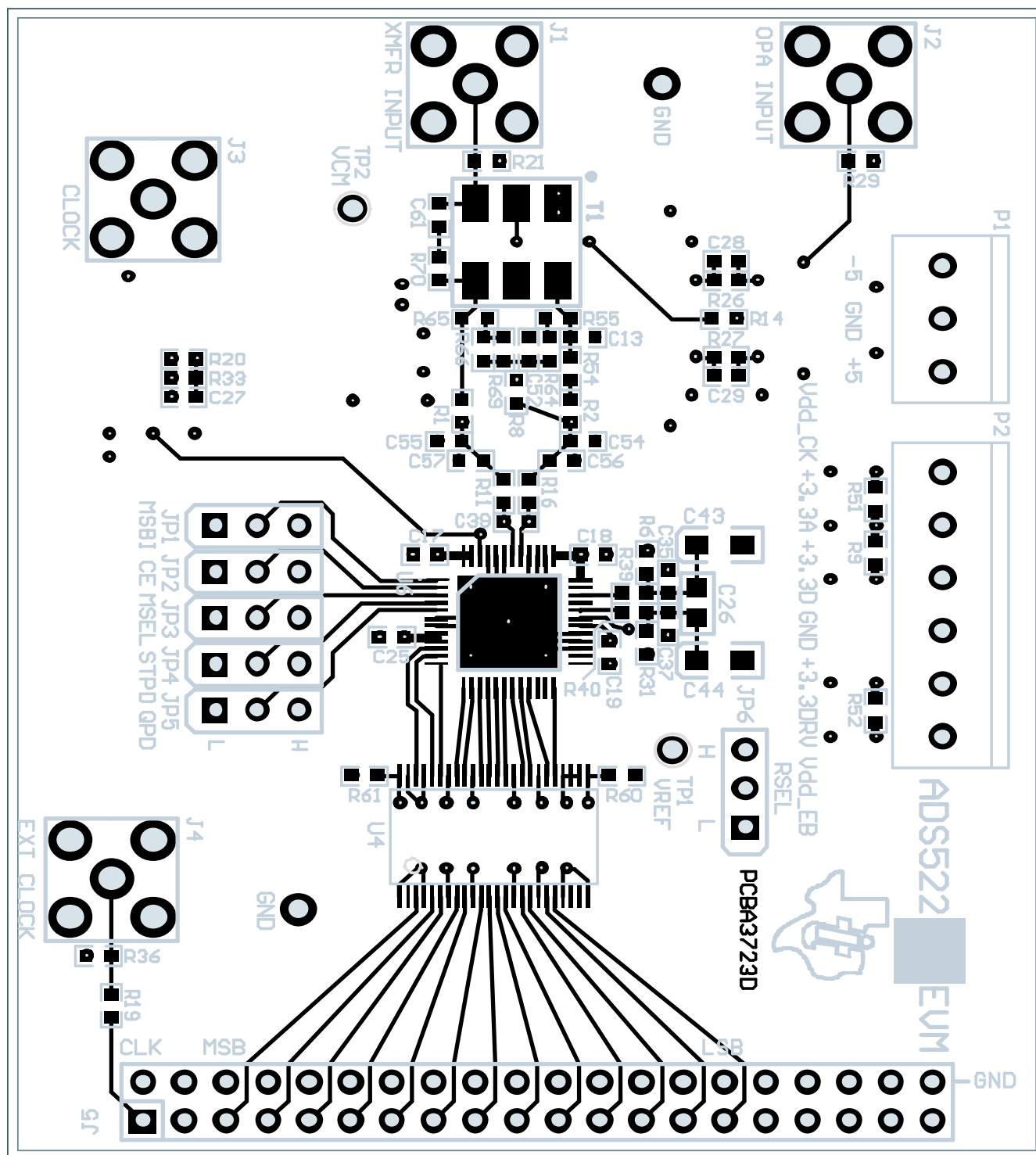
Figure 1. ADS522xEVM Top Layer
