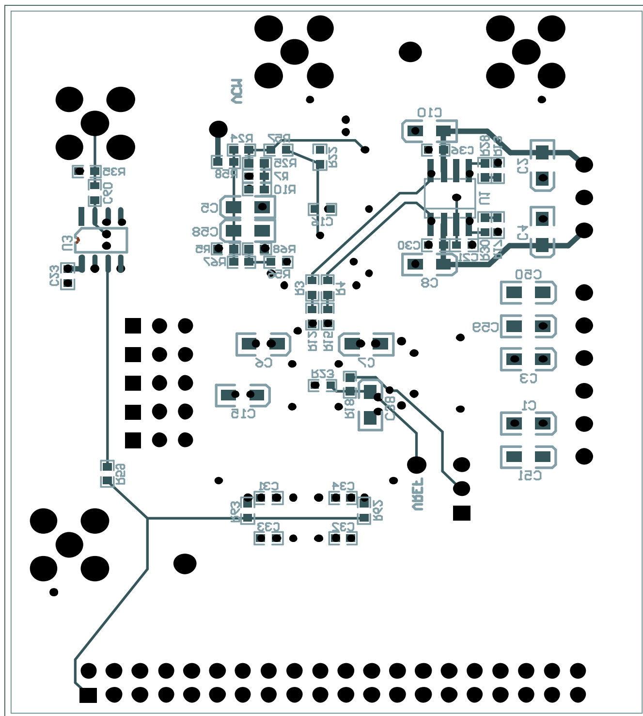
Figure 5. ADS522xEVM Bottom Layer
